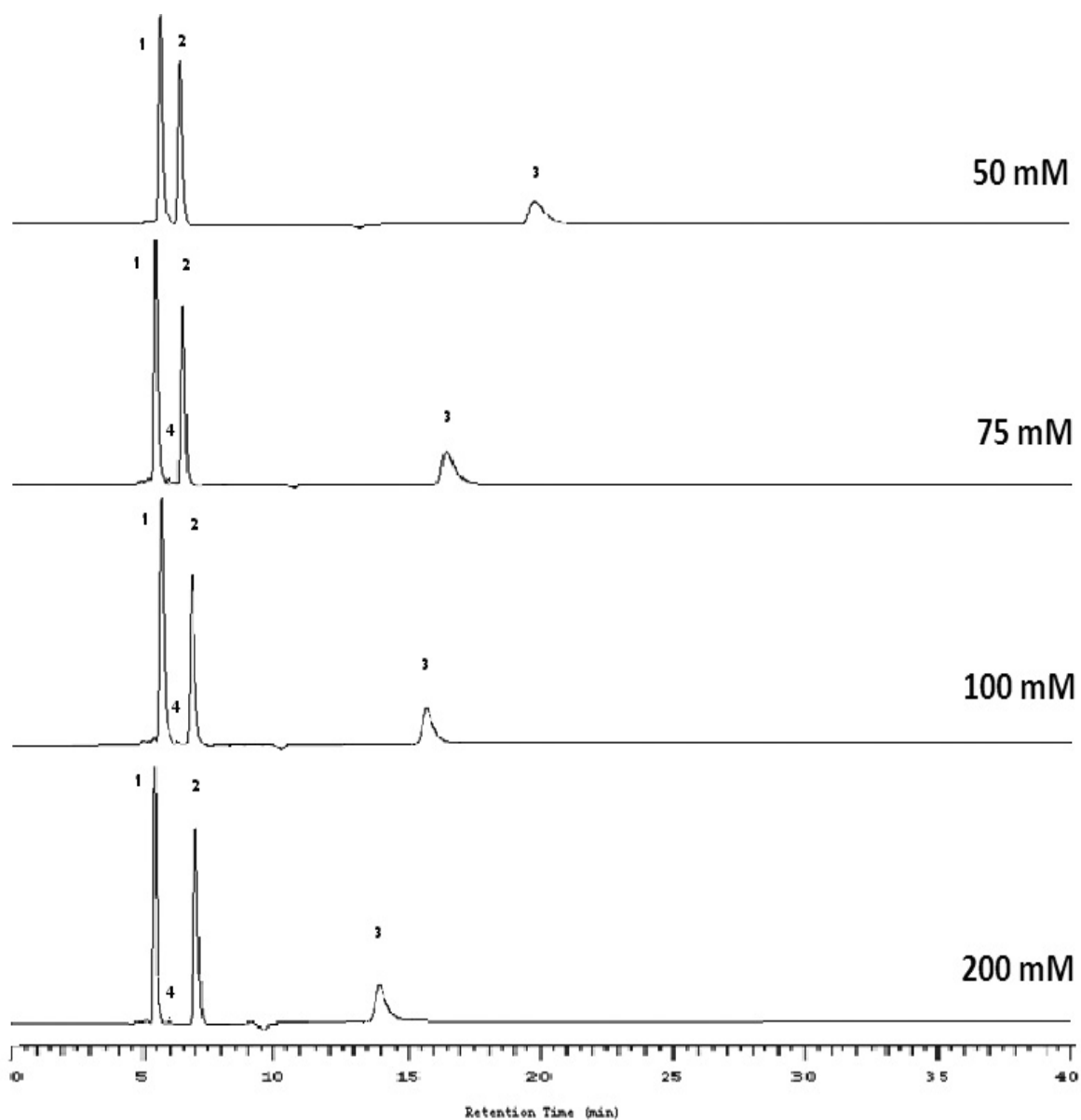
Figure (4.6): Chromatograms obtained upon 20 \mu\text{l} injection of a mixture of sulfaquinoxaline sodium (20 \mu\text{g/ml} ) (1), Vitamin \text{K}_3 (2) (10 \mu\text{g/ml} ), and amprolium hydrochloride (3) (20 \mu\text{g/ml} ), sulfaquinoxaline impurity (4). Mobile phase consisting of ACN and \text{NH}_4\text{AC} solution (80:20; v/v) adjusted to pH of 5.0; flow rate =0.5 ml/min; \lambda =263\text{nm} ; the concentration of \text{NH}_4\text{AC} is as shown in the figure.
