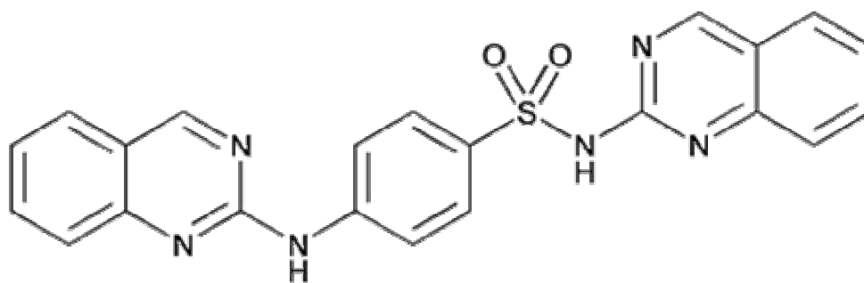
Figure (4.5): Structure of Sulfaquinoxaline Related Compound A. [55]
