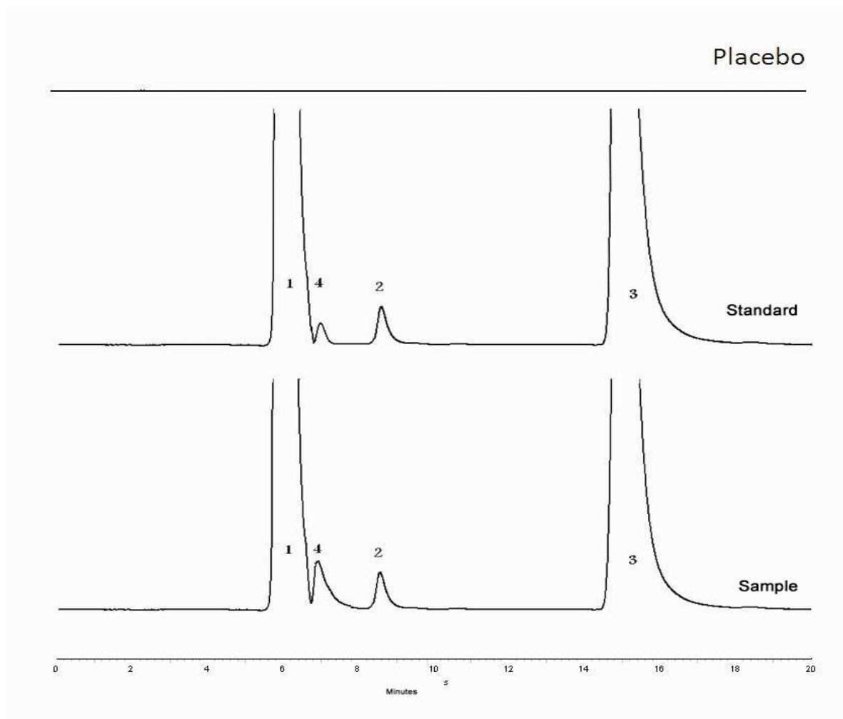
Figure (5.2): A zoomed out view chromatograms of Placebo, standard solution of sulfaquinoxaline sodium, vitamin K 3 and amprolium hydrochloride and test solution of A.S.K powder ; Column, a ZIC-HILIC column (25.0 cm long ×4.6 mm i.d.) with particle size of 5 μm protected with a ZIC-HILIC guard column (20mm× 2.1mm, 5μm); Mobile phase, acetonitrile and 0.2M ammonium acetate solution (15:85; v/v) adjusted to pH 5.7; flow rate 0.5 ml/min; λ =263nm; column temperature=25°C; Autosampler Temp. = 15°C; concentration of vitamin K 3 was about 0.2μg/ml.
