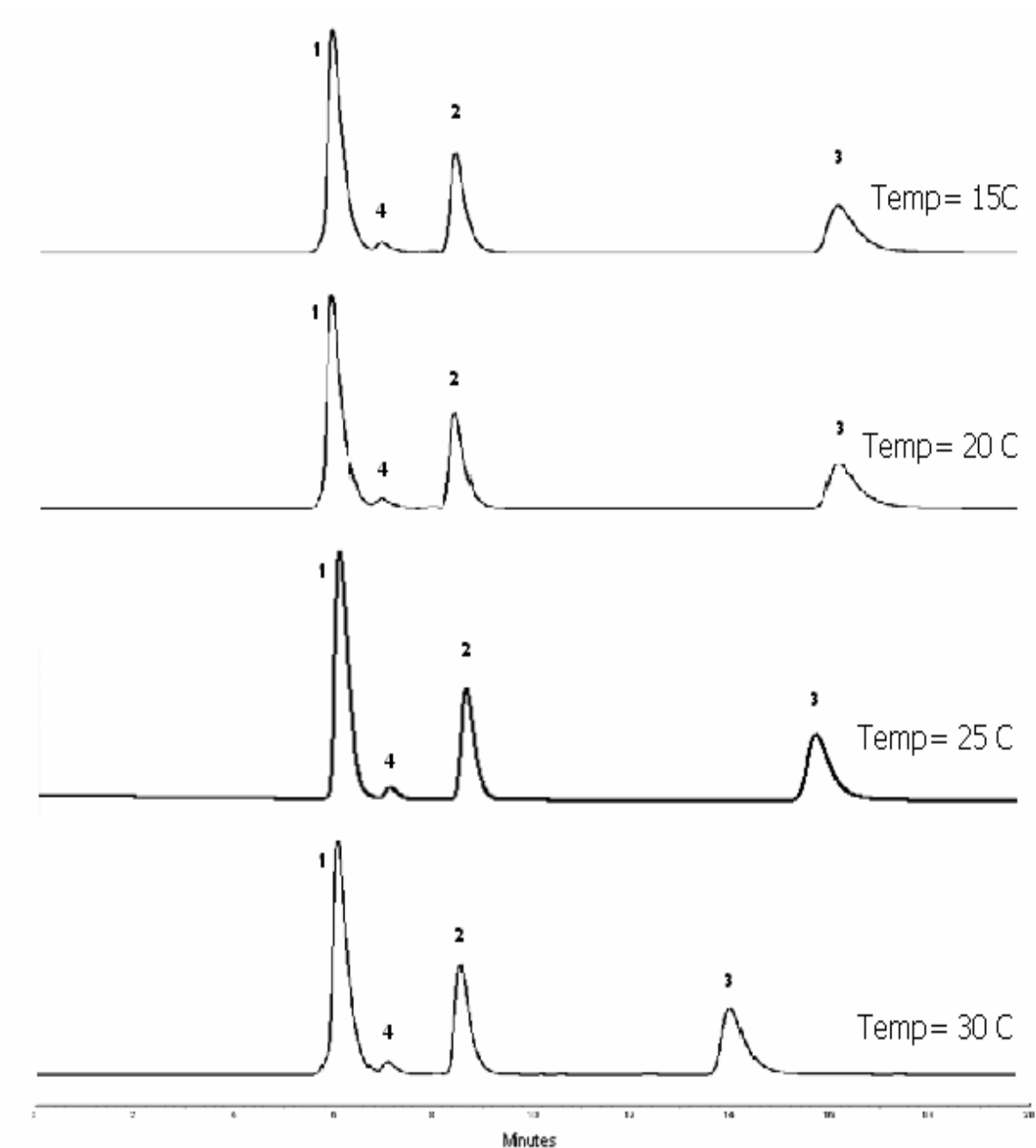
Figure (4.10): Chromatograms obtained upon 20 \mu l injection of a mixture of sulfaquinoxaline sodium (1), Vitamin K 3 (2), and amprolium hydrochloride (3), Sulfaquinoxaline impurity (4) at mobile phase consisting of ACN and 0.2M NH 4 AC solution (85:15; v/v) at pH 5.7; flow rate 0.5 ml/min; \lambda =263nm. The column temperature is as shown in the figure.
