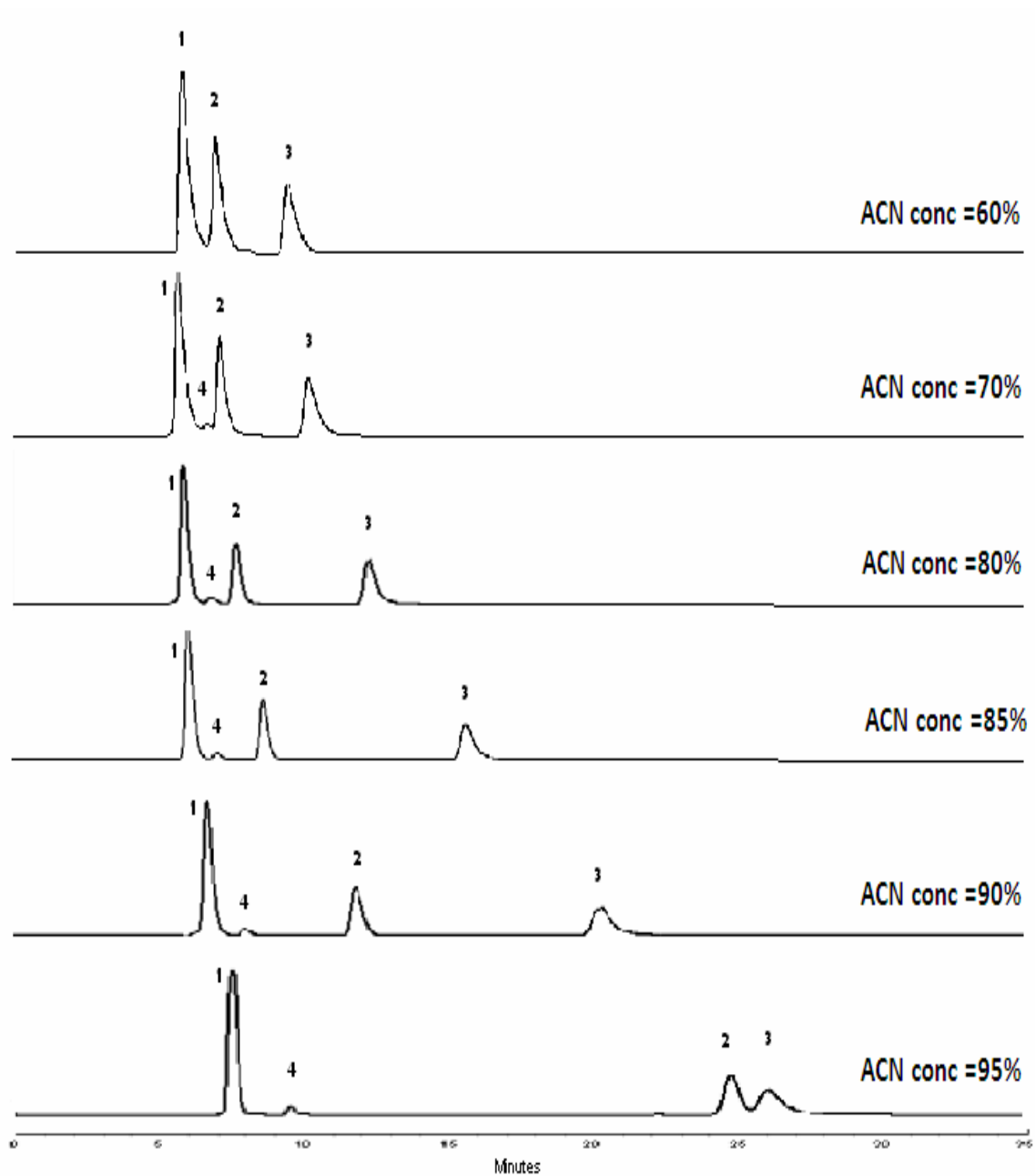
Figure (4.8): The separation obtained with 20 \mu l injection of a mixture of sulfaquinoxaline sodium (1), Vitamin K 3 (2), and amprolium hydrochloride (3), Sulfaquinoxaline impurity (4). Mobile phase consisting of ACN and 0.2M NH 4 AC solution, at pH of 5.7; flow rate 0.5 ml/min; \lambda =263nm. The %ACN is as shown in the figure.
