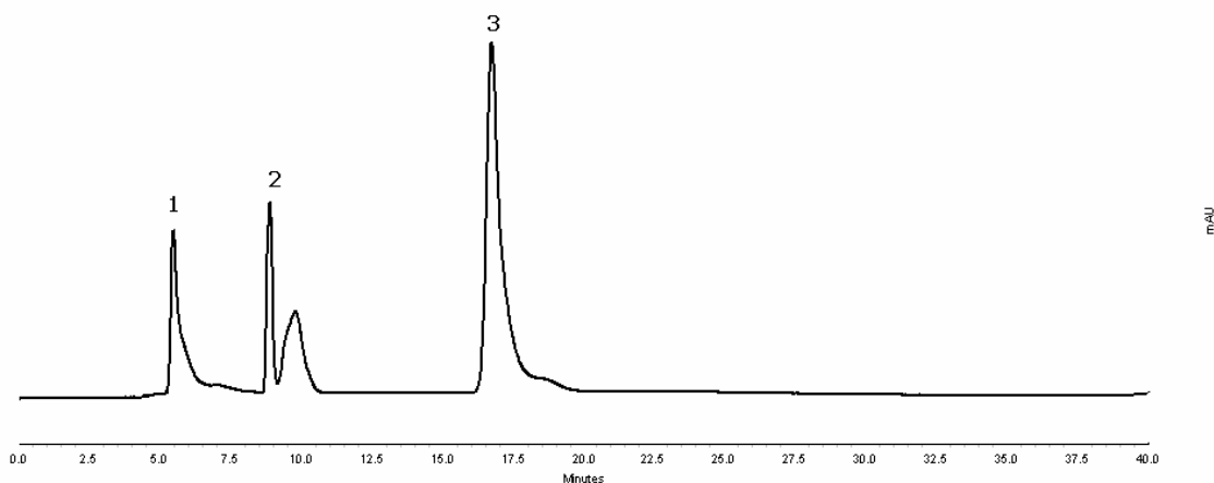
Figure (4.3): A typical chromatogram of mixture of sulfaquinoxaline sodium (3), vitamin K 3 (1) and amprolium hydrochloride (2); Column, C 8 (5 \mu m, 250mm \times 4.6mm); Mobile phase consisting of a mixture of 400 ml methanol, 600 ml water containing 1.0 g of sodium 1-decanesulfonate, 5 ml triethylamine, and 25 ml glacial acetic acid; flow rate 1.0 ml/min; \lambda =274nm; column temperature=25°C; Autosampler Temp. = 15°C.
