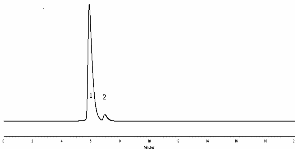
Figure (5.7): Stress test with heat for sulfaquinoxaline sodium
