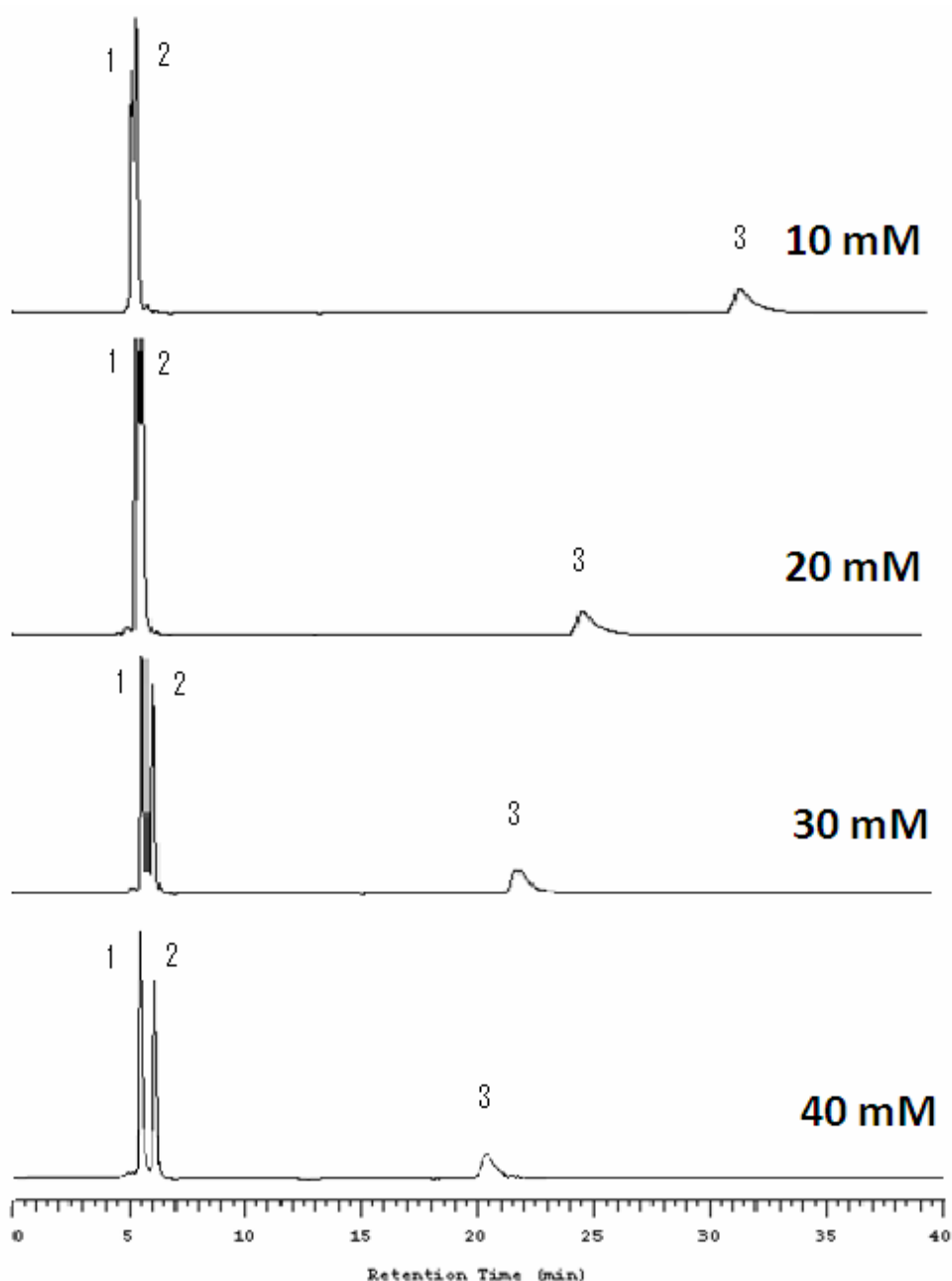
Figure (4.4): Chromatograms obtained upon 20 \mu\text{l} injection of a mixture of sulfaquinoxaline sodium (1) (20 \mu\text{g}/\text{ml} ), Vitamin \text{K}_3 (2) (10 \mu\text{g}/\text{ml} ), and amprolium hydrochloride (3) (20 \mu\text{g}/\text{ml} ). Mobile phase consisting of ACN and \text{NH}_4\text{AC} solution (80:20; v/v) adjusted to pH of 5.0; flow rate =0.5 ml/min; \lambda =263\text{nm} ; the concentration of \text{NH}_4\text{AC} is as shown in the figure.
