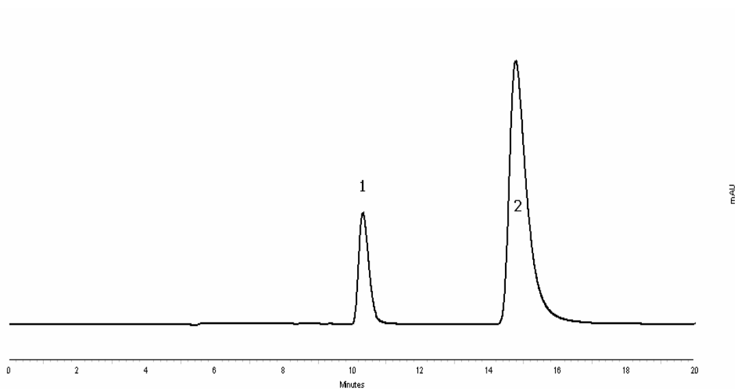
Figure (5.18): Stress test under oxidation for amprolium hydrochloride.
