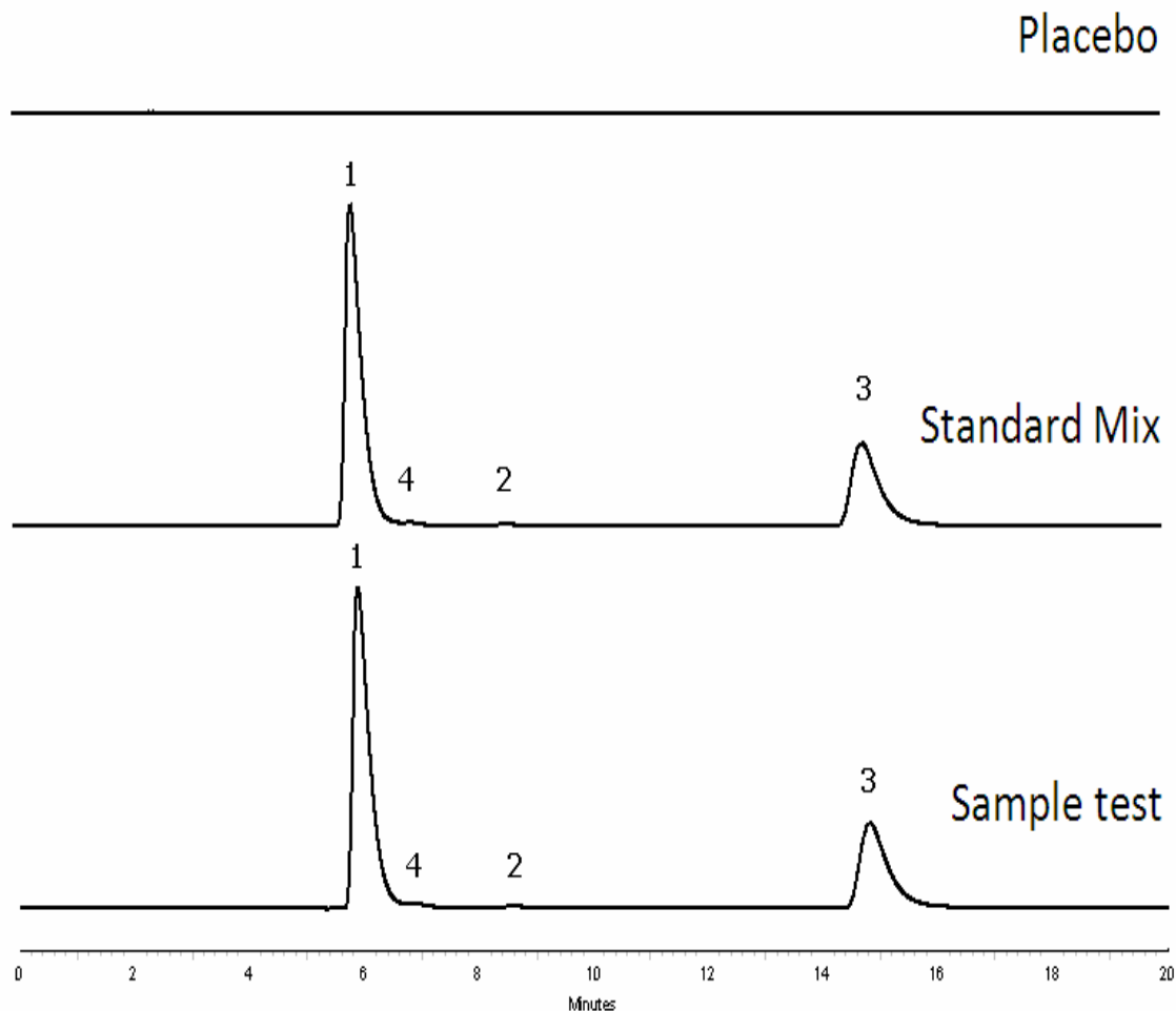
Figure (5.1): A typical chromatograms of Placebo, standard solution of sulfaquinoxaline sodium, vitamin K 3 and amprolium hydrochloride and test solution of A.S.K powder ; Column, a ZIC-HILIC column (25.0 cm long ×4.6 mm i.d.) with particle size of 5 μm protected with a ZIC-HILIC guard column (20mm× 2.1mm, 5μm); Mobile phase, acetonitrile and 0.2M ammonium acetate solution (15:85; v/v) adjusted to pH 5.7; flow rate 0.5 ml/min; λ =263nm; column temperature=25°C; Autosampler Temp. = 15°C; concentration of vitamin K 3 was about 0.2μg/ml.
