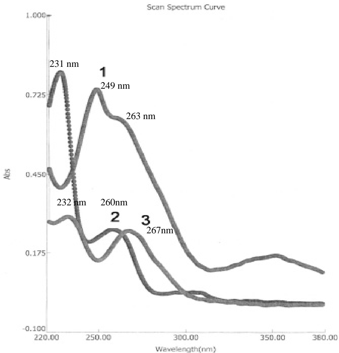
Figure (4.1): Overlaid UV-Spectra of the mixture of sulfaquinoxaline sodium (1), menadione sodium bisulfite (2) and amprolium hydrochloride (3), in the mobile phase (ACN: 0.2 M \text{NH}_4\text{AC} buffer (85:15; v/v)).
