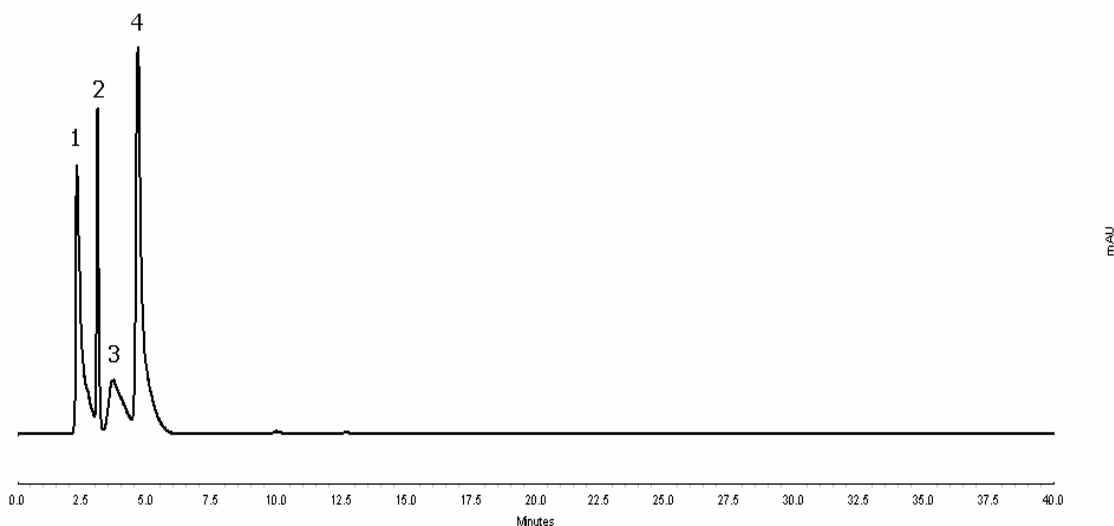
Figure (4.2): A typical chromatogram of mixture of sulfaquinoxaline sodium (4), sulfaquinoxaline related compound A (3), vitamin K 3 (1) and amprolium hydrochloride (2); Column, C 18 (5 \mu m, 250mm \times 4.6mm) ; Mobile phase consisting of 2.0 g of sodium 1-hexanesulfonate in 500 ml of water; 12 ml of glacial acetic acid, 2.0 ml of triethylamine, 450 ml of methanol and 50 ml of acetonitrile; flow rate 1.0 ml/min; \lambda =274nm; column temperature=25°C; Autosampler Temp.= 15°C.
