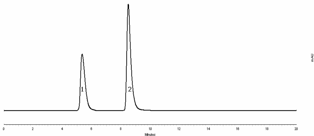
Figure (5.12): Stress test with heat for menadione sodium bisulfite.
