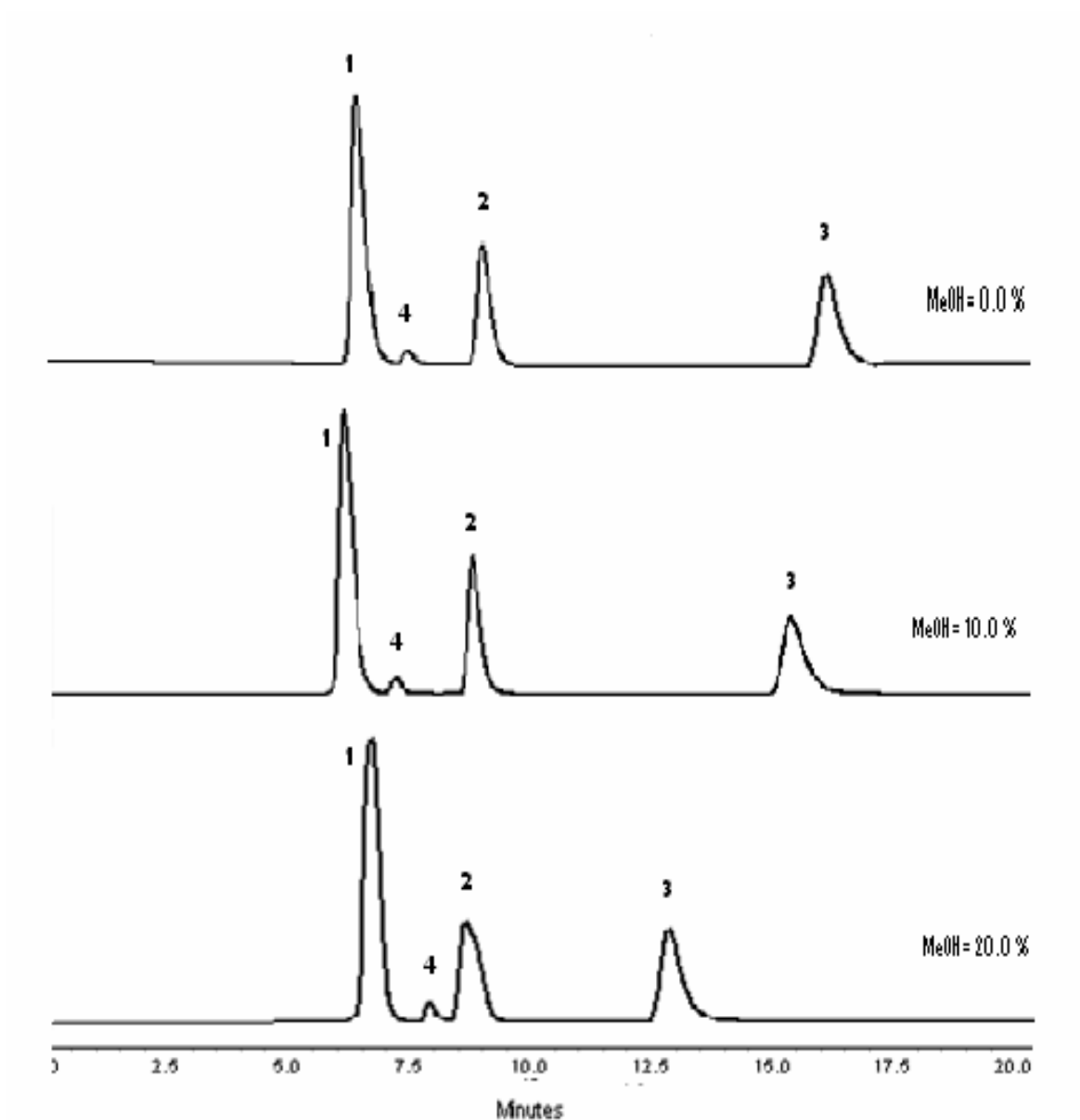
Figure (4.9): The separation obtained with 20 \mu l injection of a mixture of sulfaquinoxaline sodium (1), Vitamin K 3 (2), and amprolium hydrochloride (3), Sulfaquinoxaline impurity (4) at mobile phase consisting of MeOH with ACN and 0.2 M NH 4 AC (10 :75 :15; v/v/v ) at pH of 5.7 and MeOH with ACN and 0.2 M NH 4 AC (20 :65 :15; v/v/v ) at pH of 5.7, respectively; flow rate 0.5 ml/min; \lambda =263nm.
