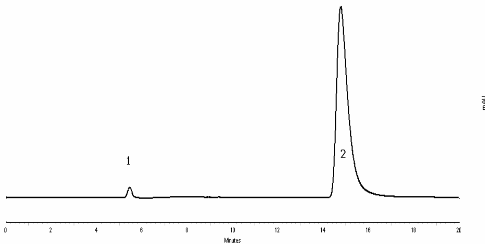
Figure (5.20): Stress test with hydrochloric acid for amprolium hydrochloride.
