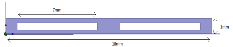
Fig. 8 (a) Geometries of MIMO antenna with vertical stub.
