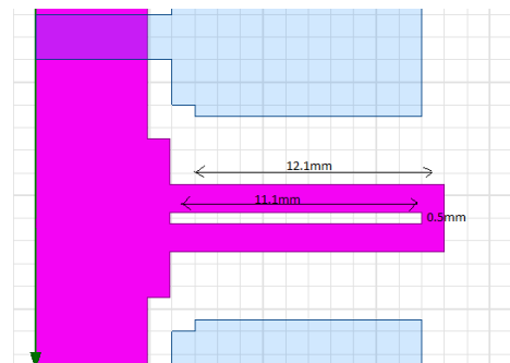
Fig. 10 Geometries of the ground stub.
