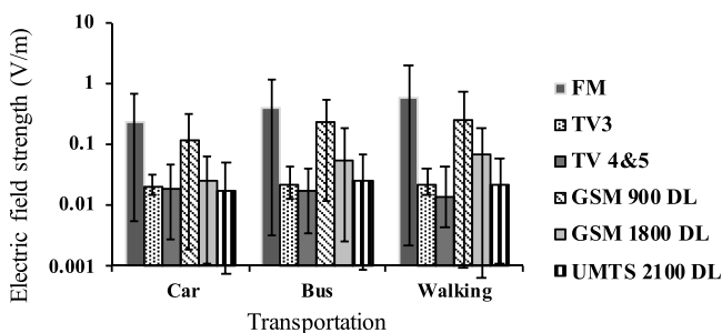
Fig. 3. Mean exposure to 24 participants from fixed outdoor RF-EMF sources during different transportation modes.
