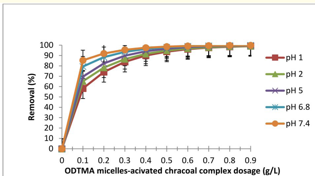
Figure 2: Effect of pH and adsorbent dosage on the percent removal of paracetamol by OMAC complex. Initial concentration of paracetamol = 50 ppm, contact time = 4h, temperature = 25.0°C.
