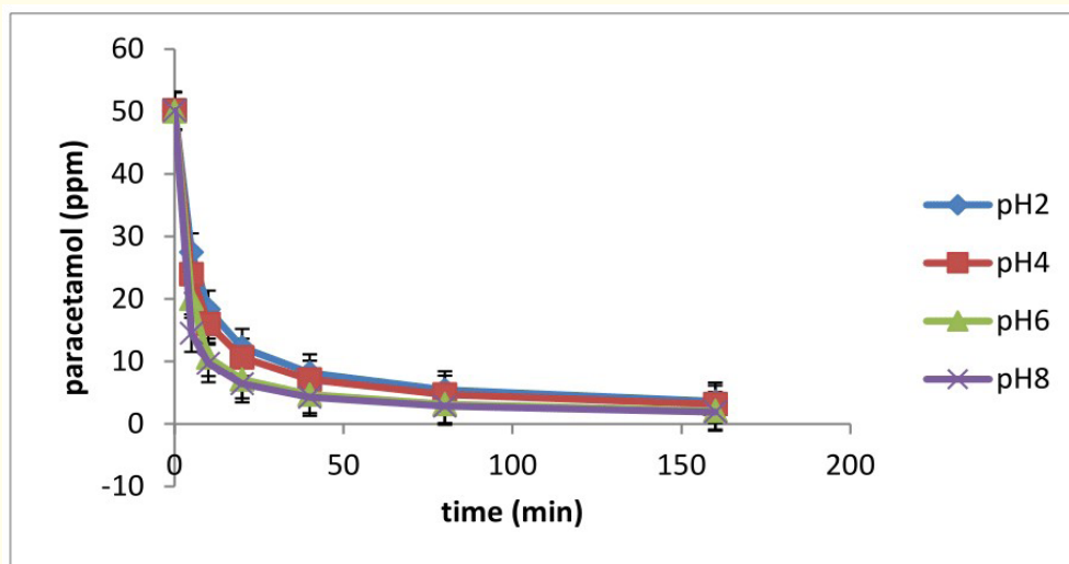
Figure 3: Effect of contact time on the adsorption of paracetamol onto activated charcoal at different pH. Temperature = 25.0°C and activated charcoal dosage = 0.5 g/L.
