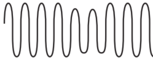
Figure 2.4: Voltage sag.
