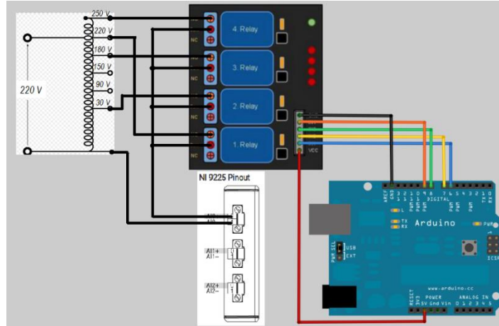
Figure 4.2: Schematic diagram of Programmable ac source.
