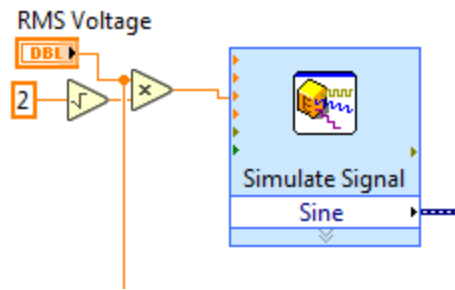
Figure B.2: Simulate signal VI.
