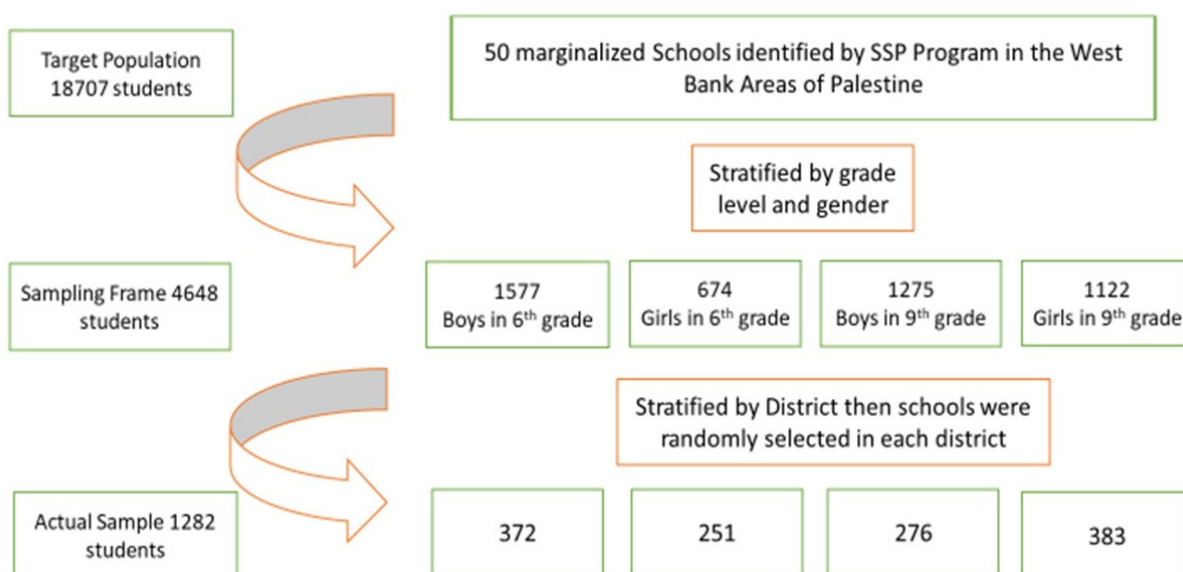
Figure 2. Flow chart about the stratified cluster sampling technique used in this study
