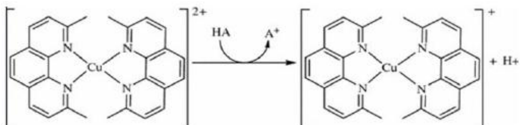
Figure 1.6: CUPRAC reaction by an oxidation molecule (HA: an antioxidant molecule, \text{A}^+ : an oxidized antioxidant molecule) (Tütem et al , 1991).
