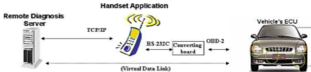
Figure 2.8: Configuration of the proposed vehicle diagnostic system.
