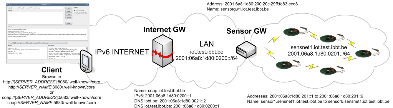
Figure 8. Publicly reachable testbed at IBTT
