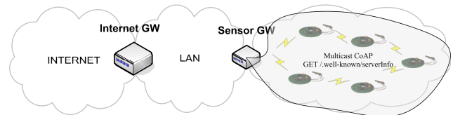
Figure 2. Discovery of sensor nodes by the sensor gateway by sending a CoAP multicast GET request for /.well-known/serverInfo in the sensor network
