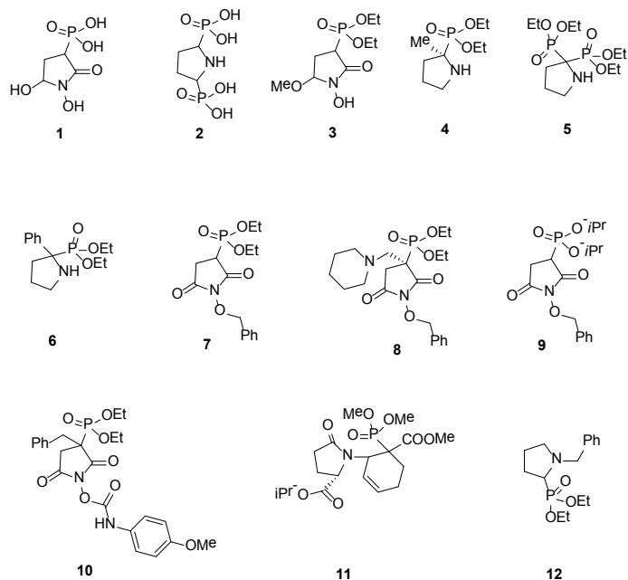
Figure 1. Pyrrolidinyl phosphonates 1-12 .
