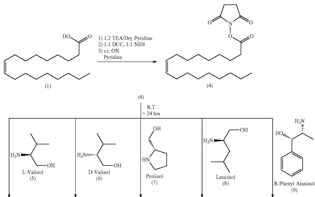
Scheme -2: Synthesis of Oleoyl-Derivatives: Oleoyl-L-Valinol (10), -D-Valinol (11), -L-Prolinol (12), -L-Leucinol (13), R-Phenyl Alaninol (14)
