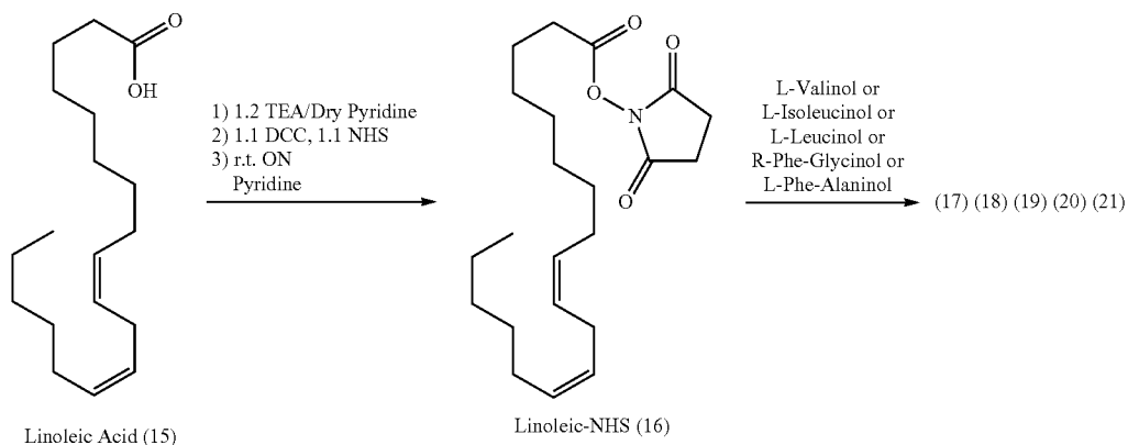
Scheme-3: Synthesis of Linoleic-Amino-OI Derivatives (17-21)
