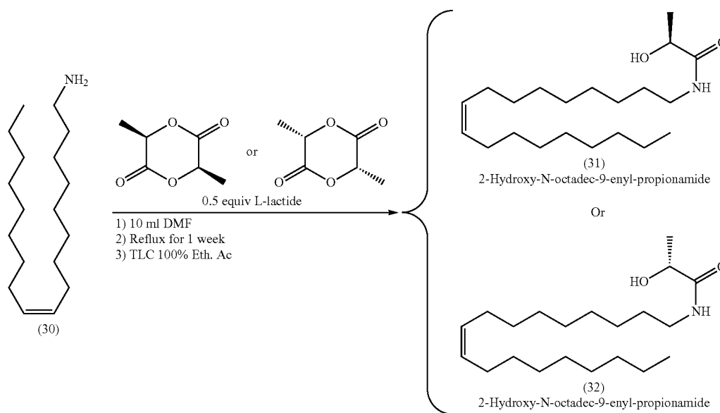
Scheme-5: Synthesis of the oleoyl-lactides (31) and (32).
